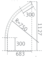
Drawing refers to 60° bowed track
