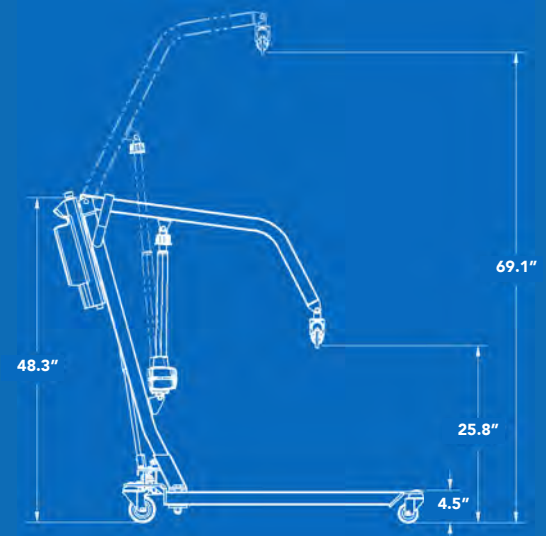
SIDE VIEW OF PL273
