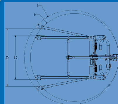
TOP VIEW OF PL400EF
